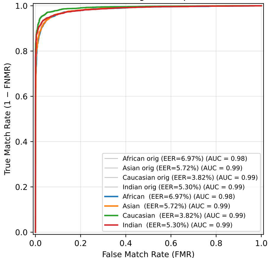
ROC — Brightness ( \beta=1 )
