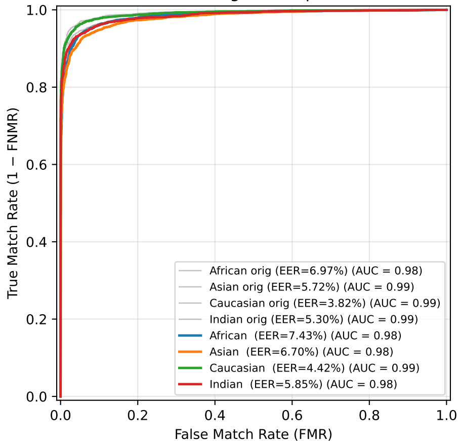
ROC — Brightness ( \beta=1.2 )
