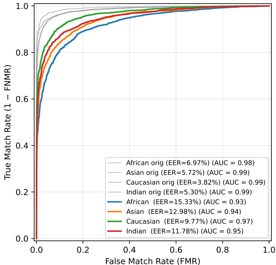
ROC — Gaussian Blur ( \sigma=2 )
