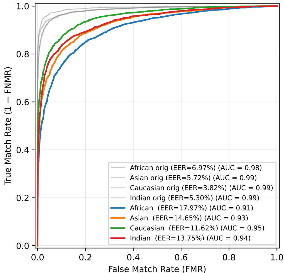
ROC — Gaussian Blur ( \sigma=2.2 )
