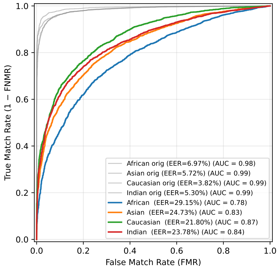
ROC — Gaussian Blur ( \sigma=3.4 )
