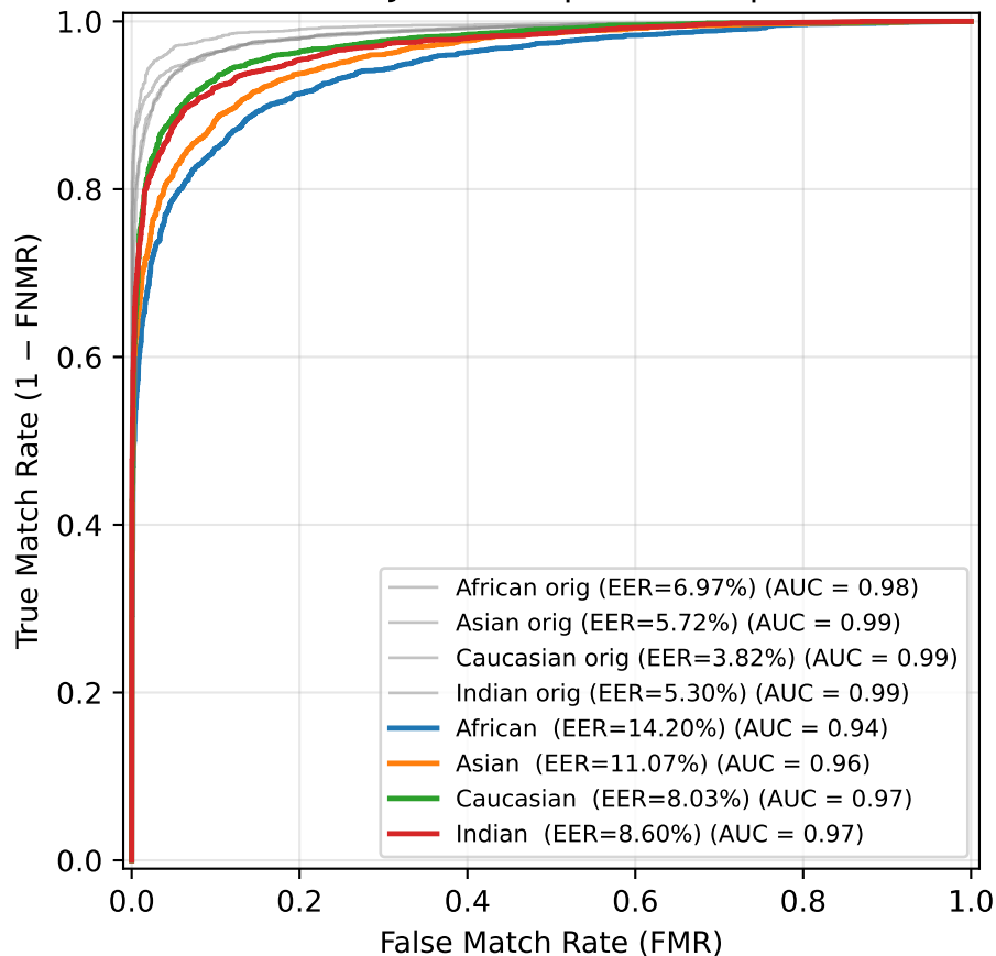
ROC — JPEG Compression (q=20)
