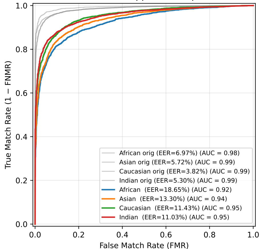
ROC — Salt & Pepper Noise (p=0.03)
