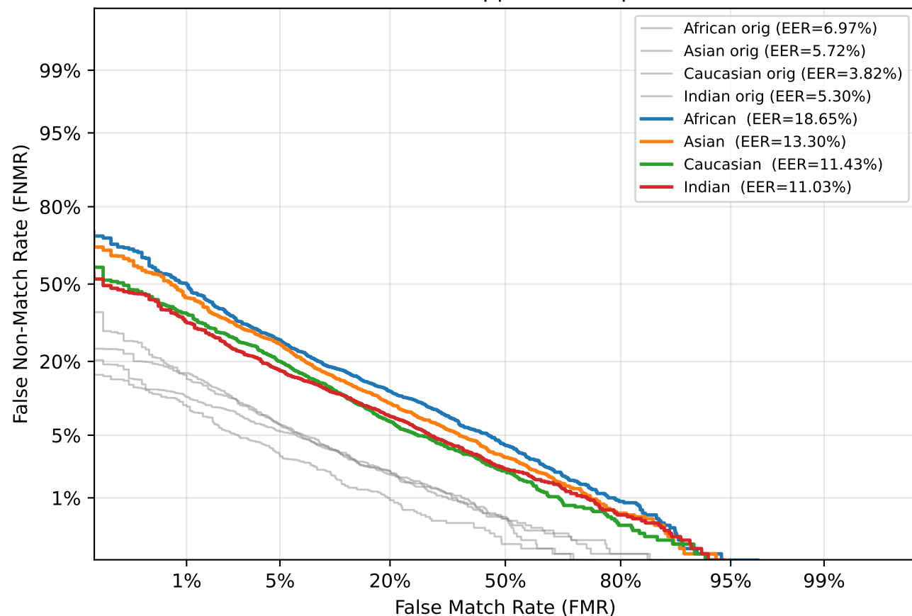
DET — Salt & Pepper Noise (p=0.03)
