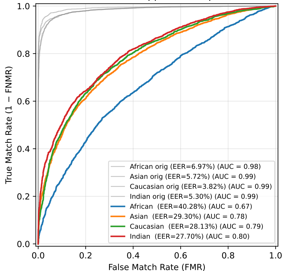
ROC — Salt & Pepper Noise (p=0.15)
