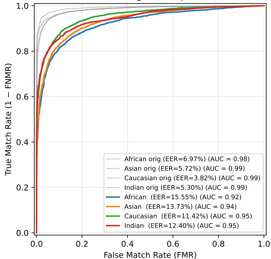
ROC — Brightness ( \beta=0.1 )
