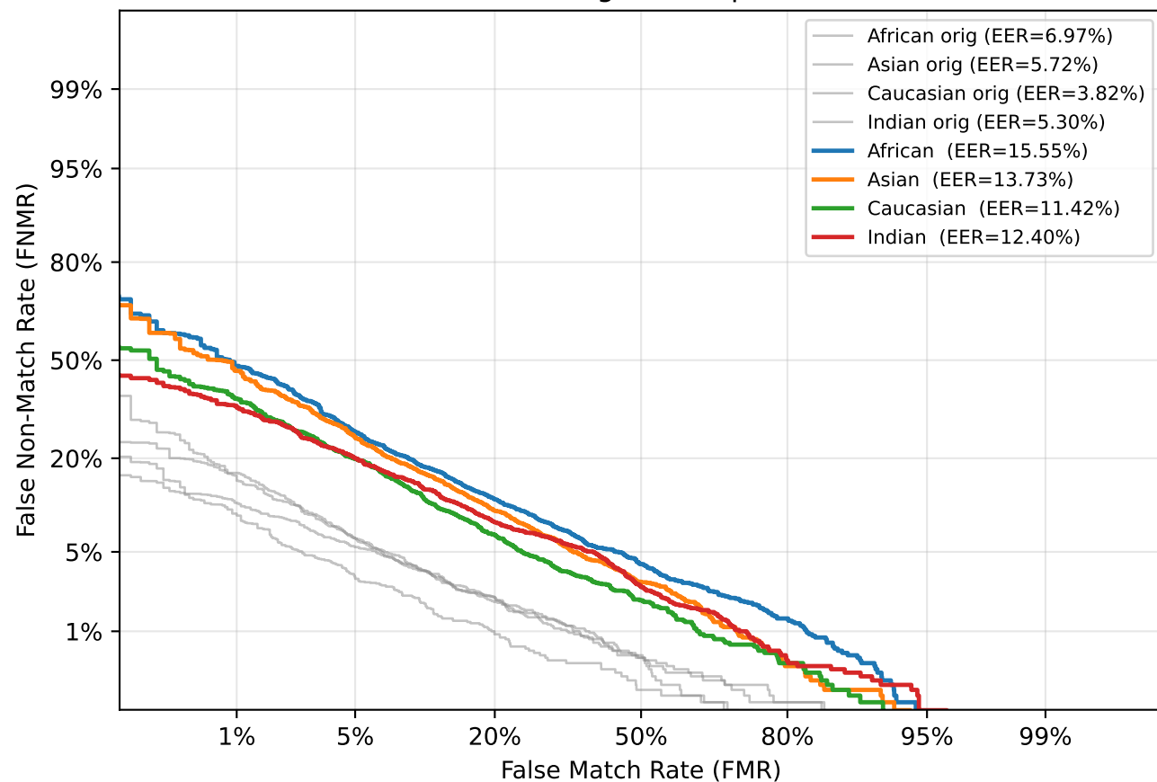
DET — Brightness ( \beta=0.1 )
