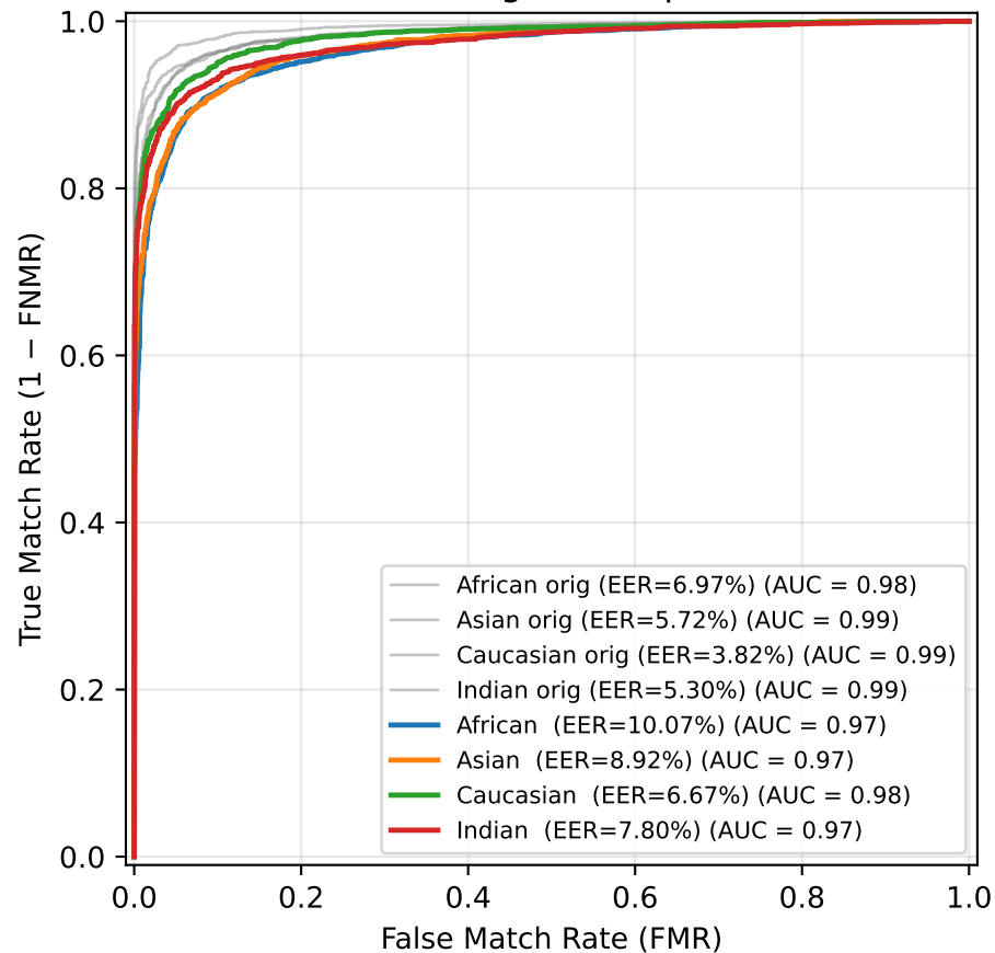
ROC — Brightness ( \beta=0.2 )
