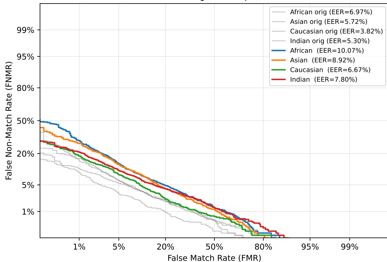
DET — Brightness ( \beta=0.2 )
