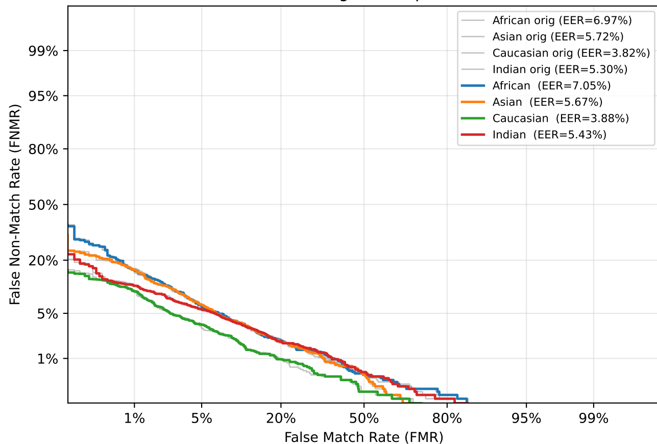
DET — Brightness ( \beta=0.9 )
