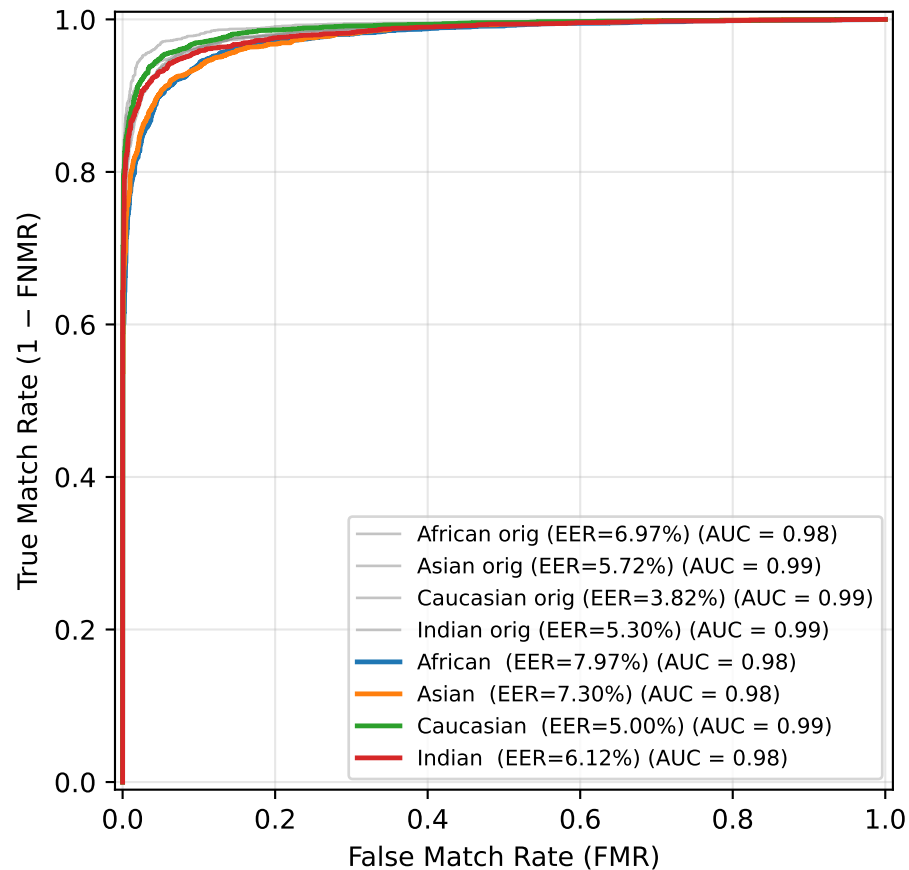
ROC — Contrast ( \alpha=0.4 )
