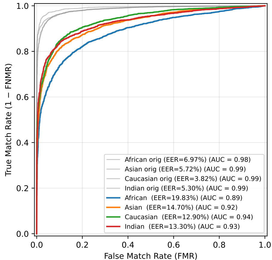
ROC — Contrast ( \alpha=3 )
