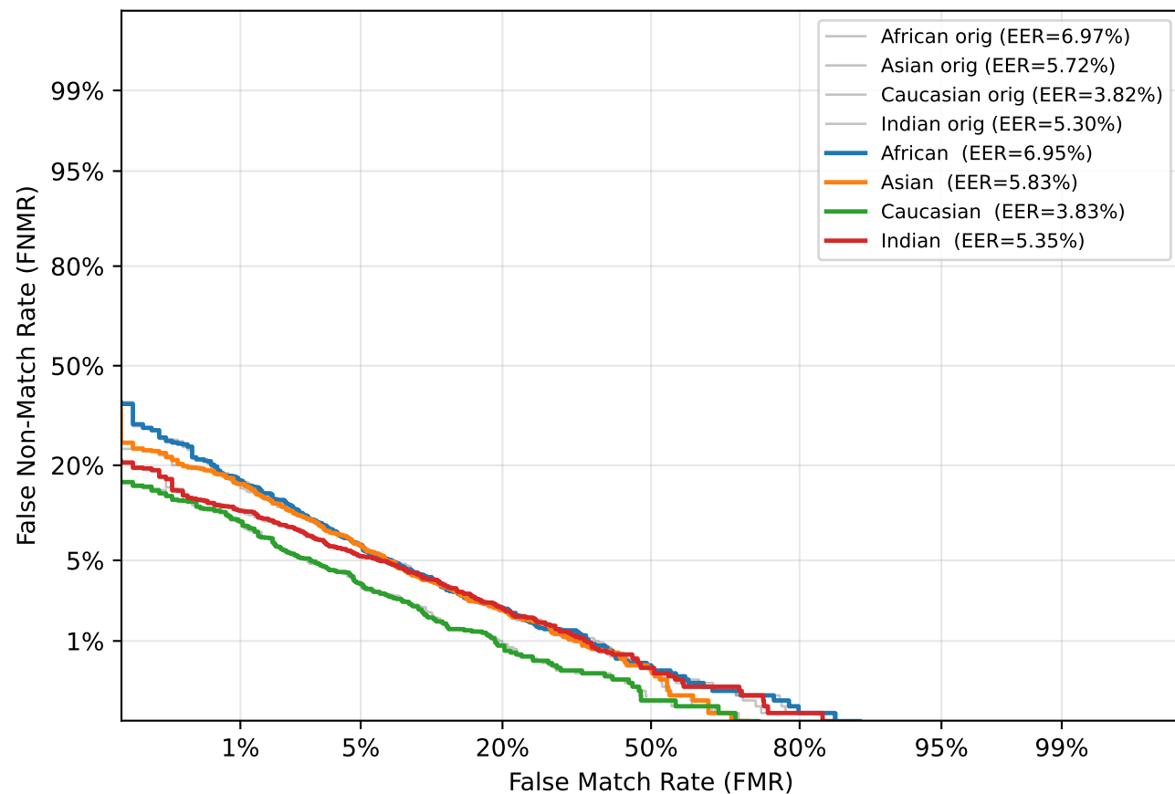
DET — Gaussian Blur ( \sigma=0.4 )
