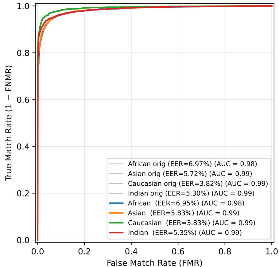
ROC — Gaussian Blur ( \sigma=0.4 )
