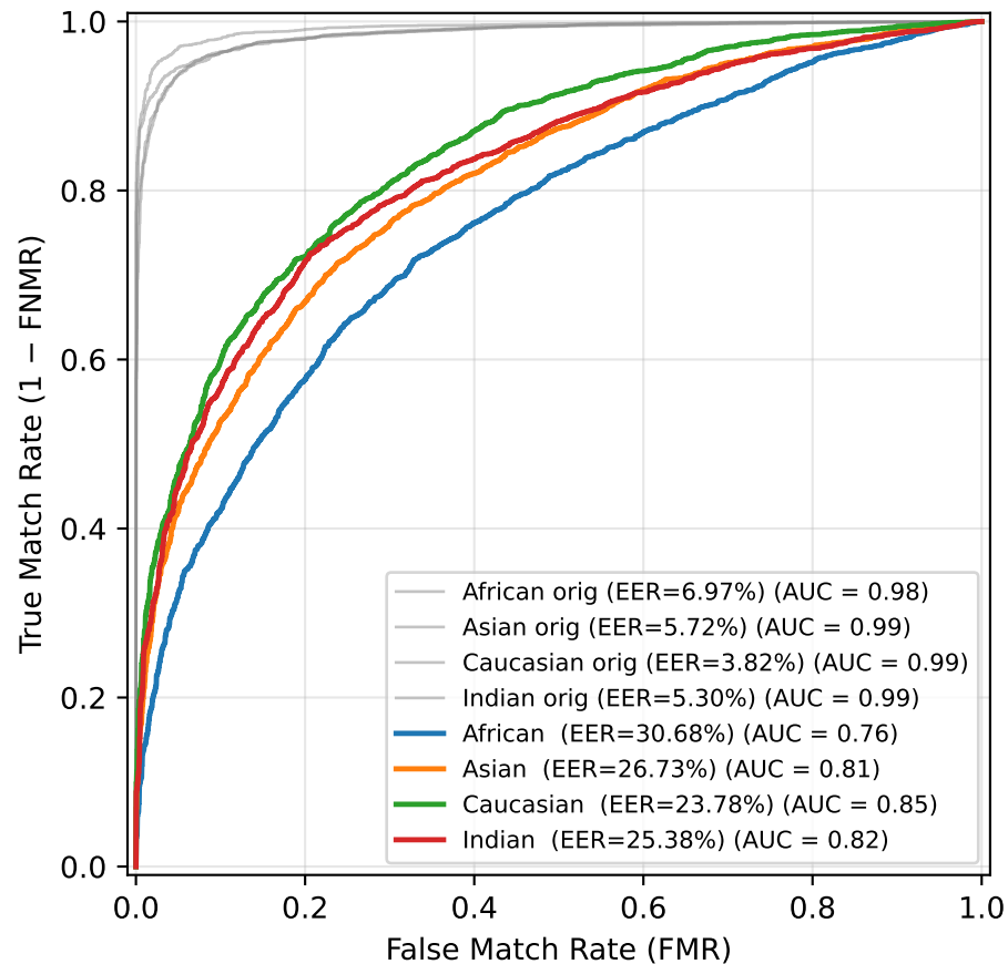
ROC — Gaussian Blur ( \sigma=3.6 )
