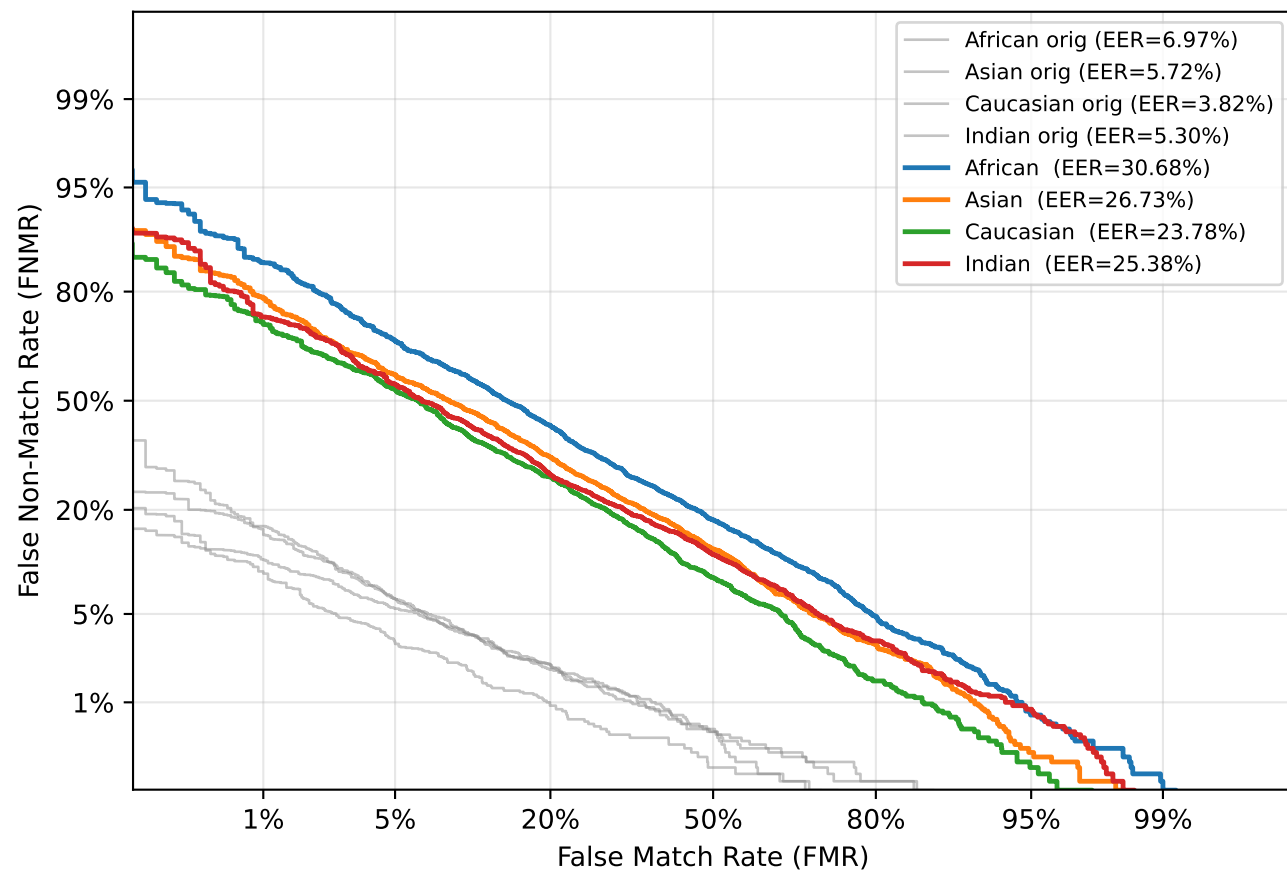
DET — Gaussian Blur ( \sigma=3.6 )
