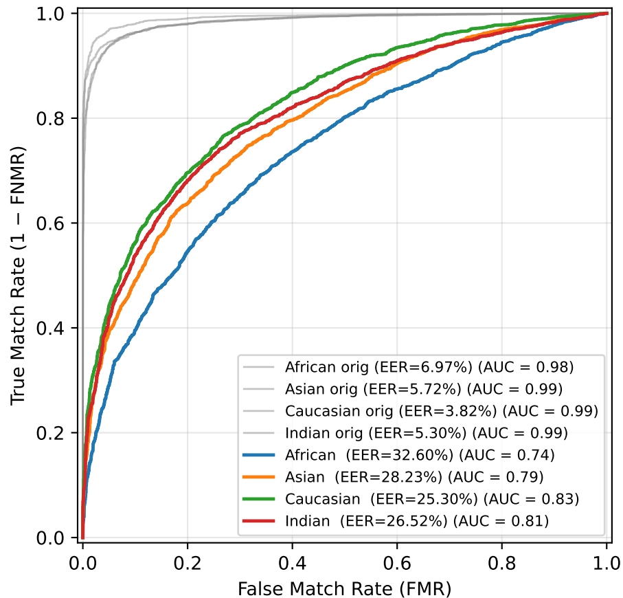
ROC — Gaussian Blur ( \sigma=3.8 )
