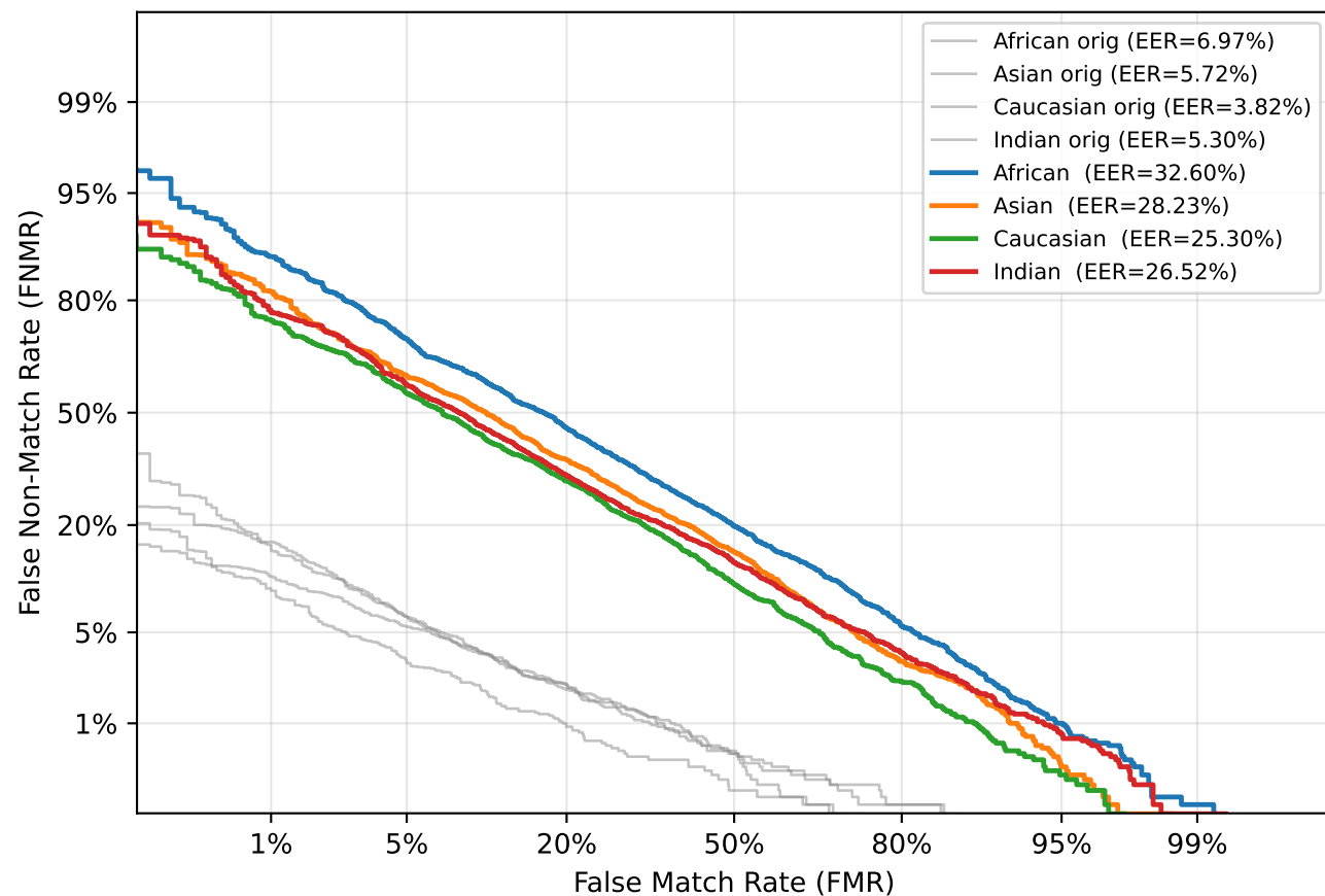
DET — Gaussian Blur ( \sigma=3.8 )
