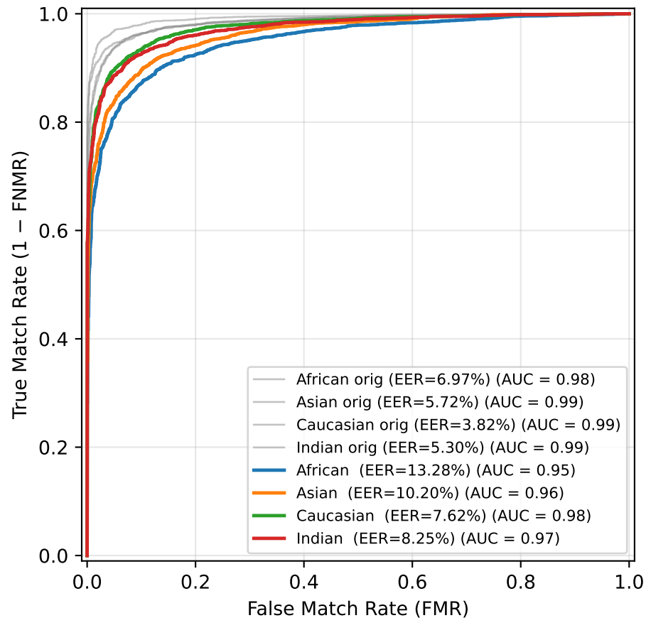
ROC — Gaussian Noise ( \sigma=10 )
