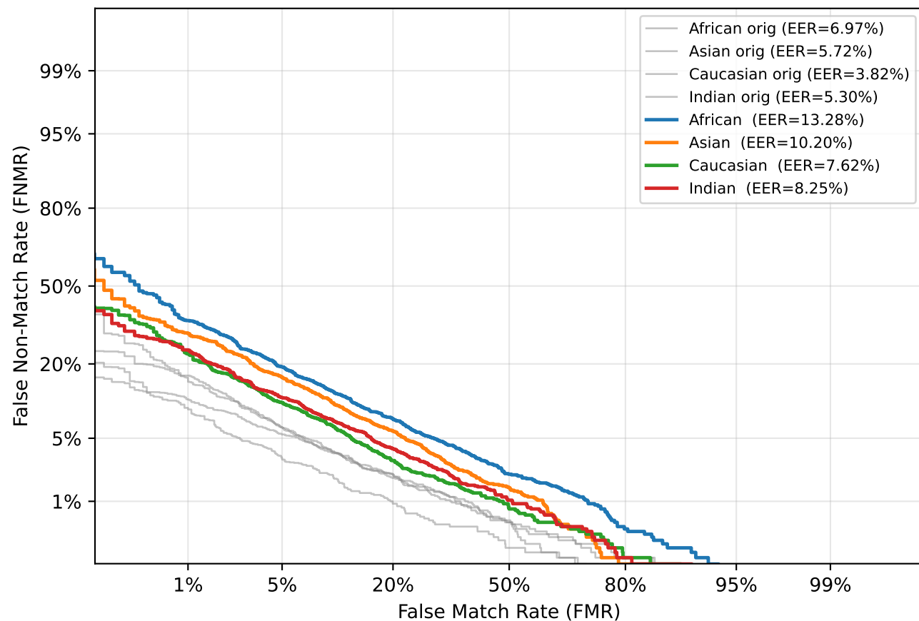
DET — Gaussian Noise ( \sigma=10 )
