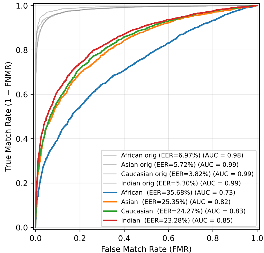
ROC — Gaussian Noise ( \sigma=40 )
