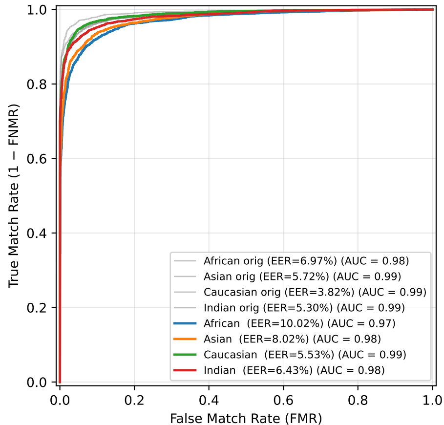
ROC — Gaussian Noise ( \sigma=6 )
