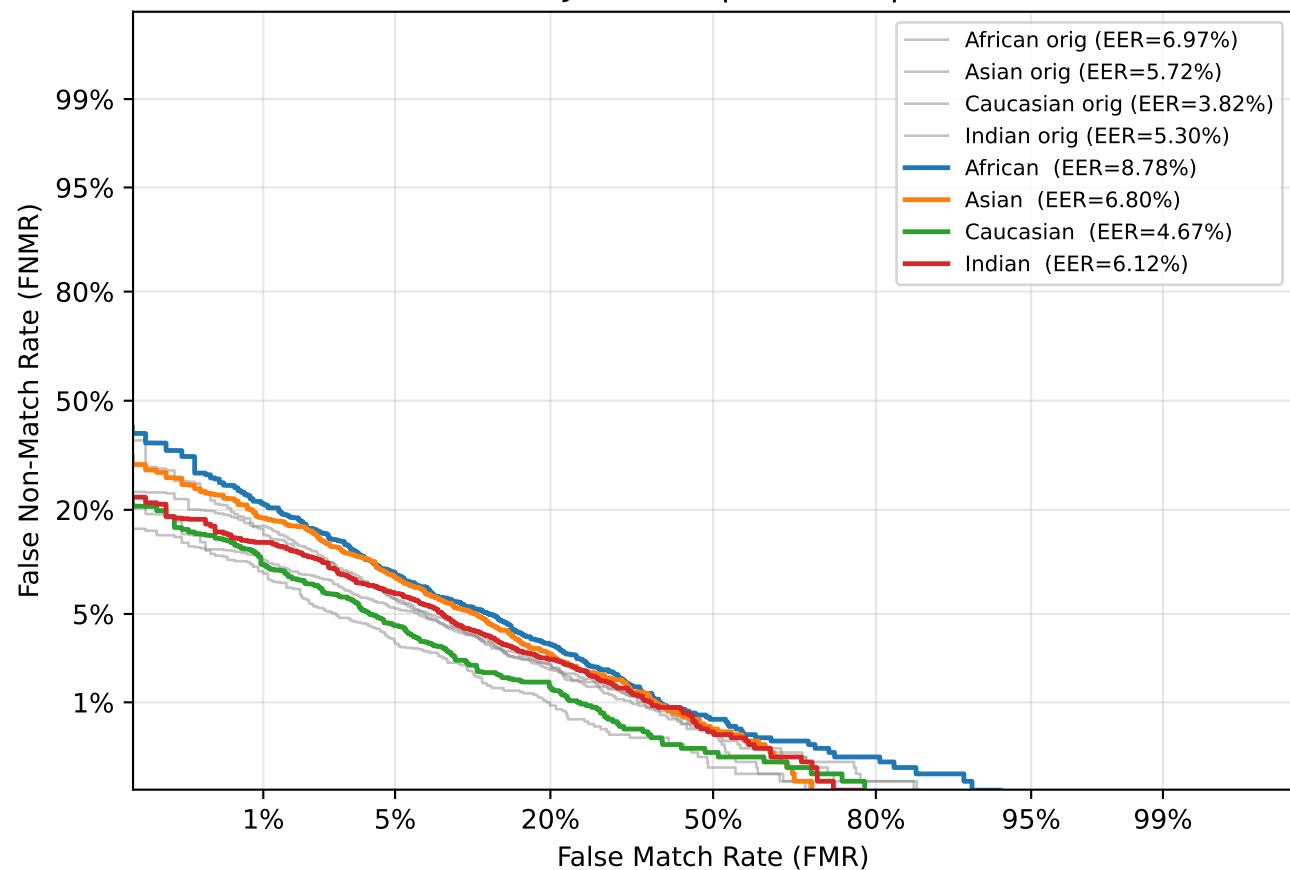
DET — JPEG Compression (q=60)
