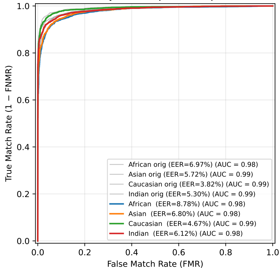
ROC — JPEG Compression (q=60)
