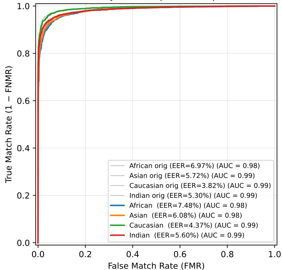
ROC — JPEG Compression (q=80)
