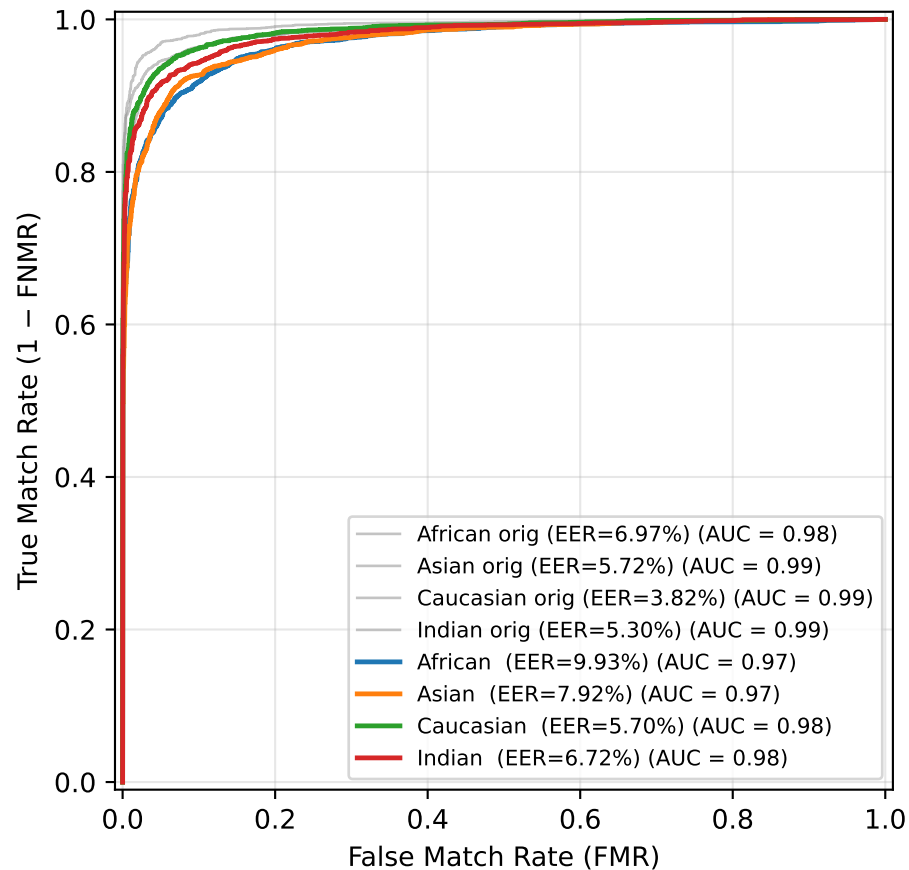
ROC — Motion Blur (k=5)
