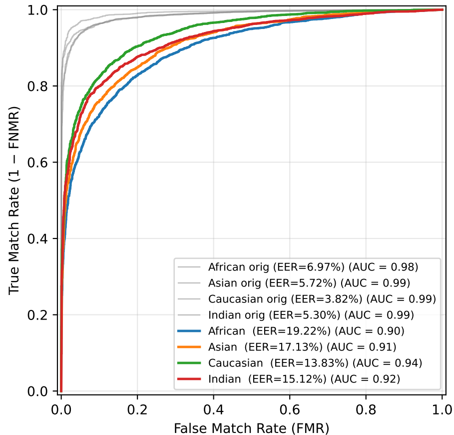
ROC — Motion Blur (k=9)
