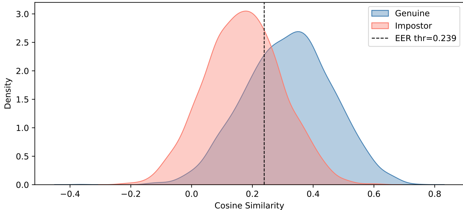
Asian — Salt & Pepper Noise (p=0.15)
