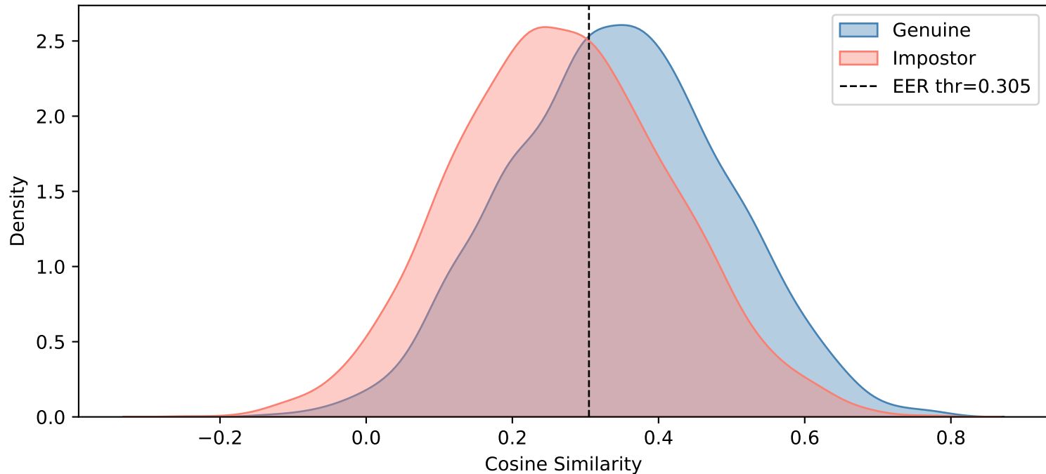
Asian — Salt & Pepper Noise (p=0.27)
