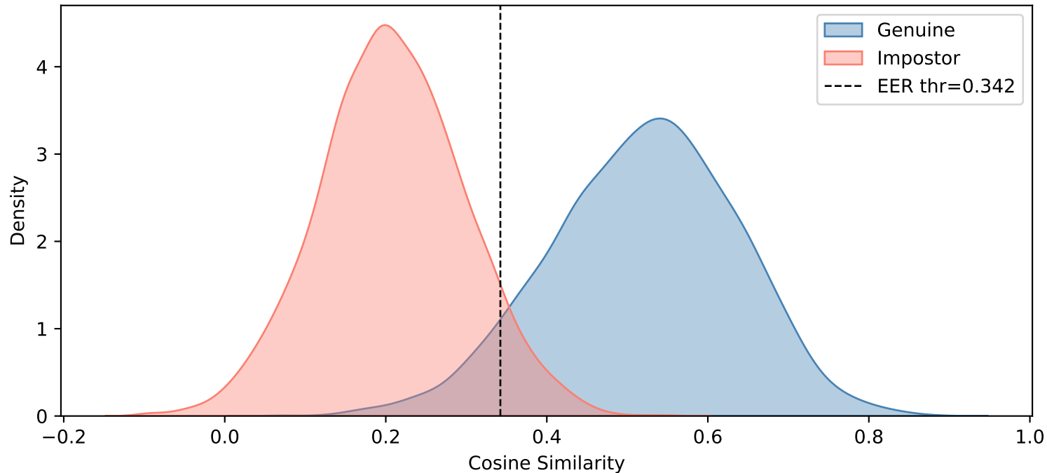
Asian — JPEG Compression (q=60)
