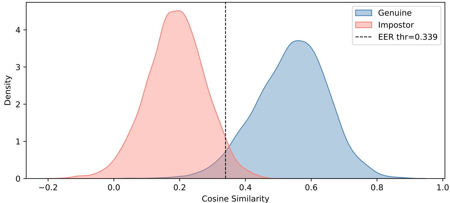
Caucasian — Contrast ( \alpha=1 )
