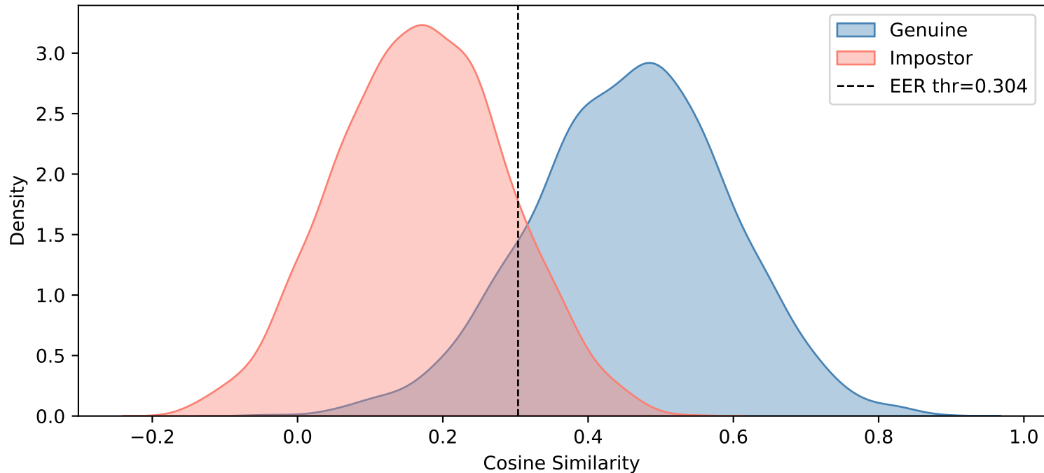
Caucasian — Gaussian Blur ( \sigma=2.4 )
