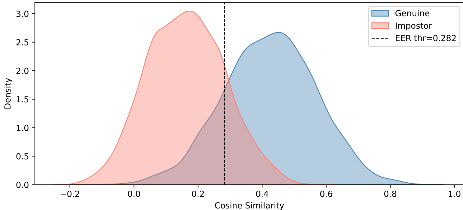
Caucasian — Gaussian Blur ( \sigma=2.8 )
