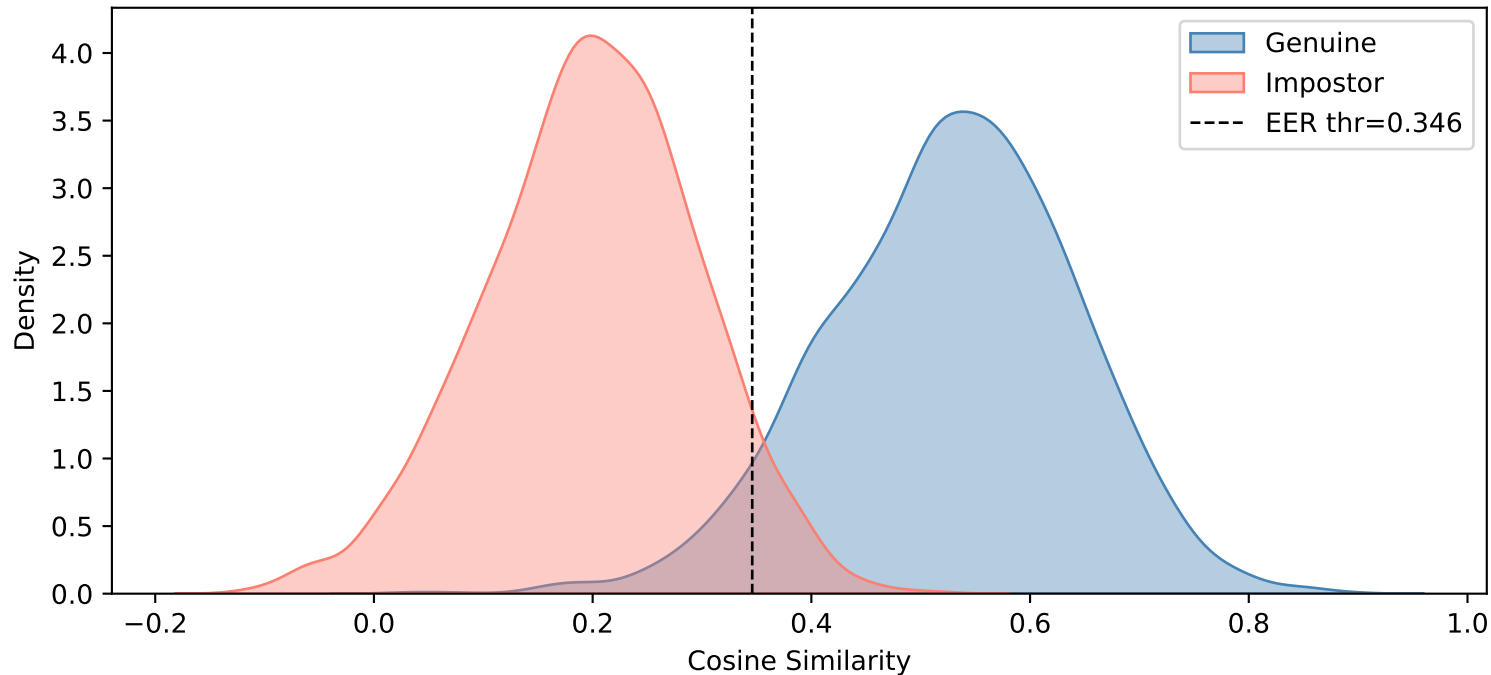
Caucasian — Motion Blur (k=5)
