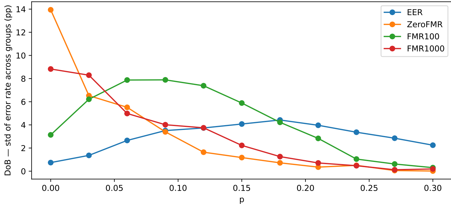
Degree of Bias — Salt & Pepper Noise
