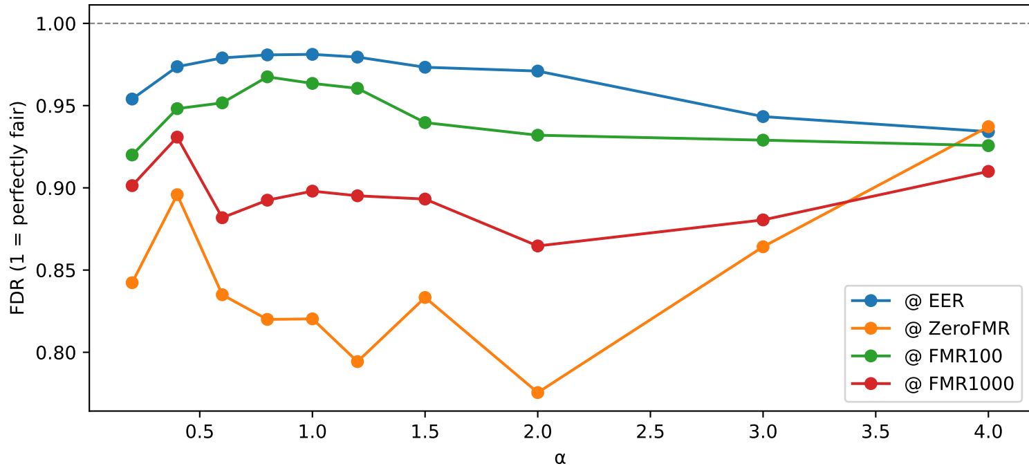
FDR — Contrast
