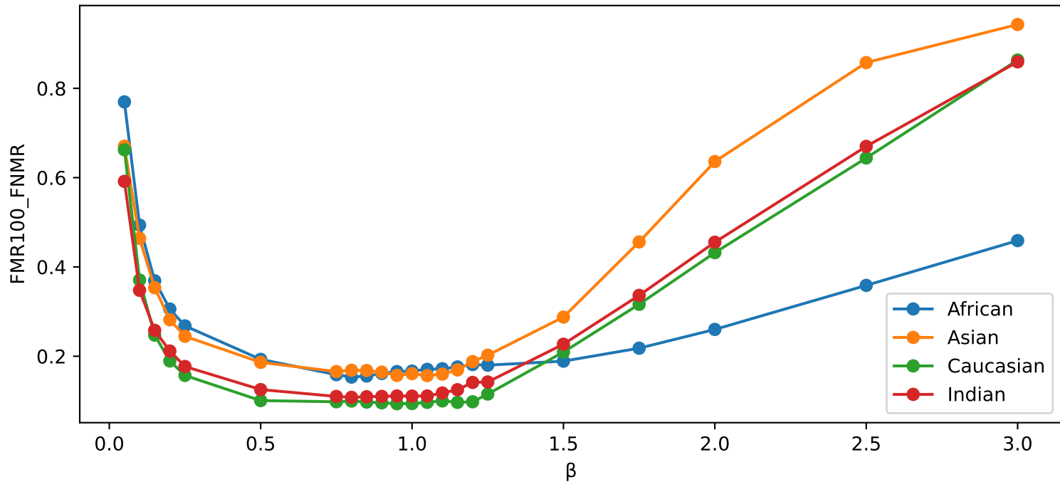
FMR100_FNMR — Brightness
