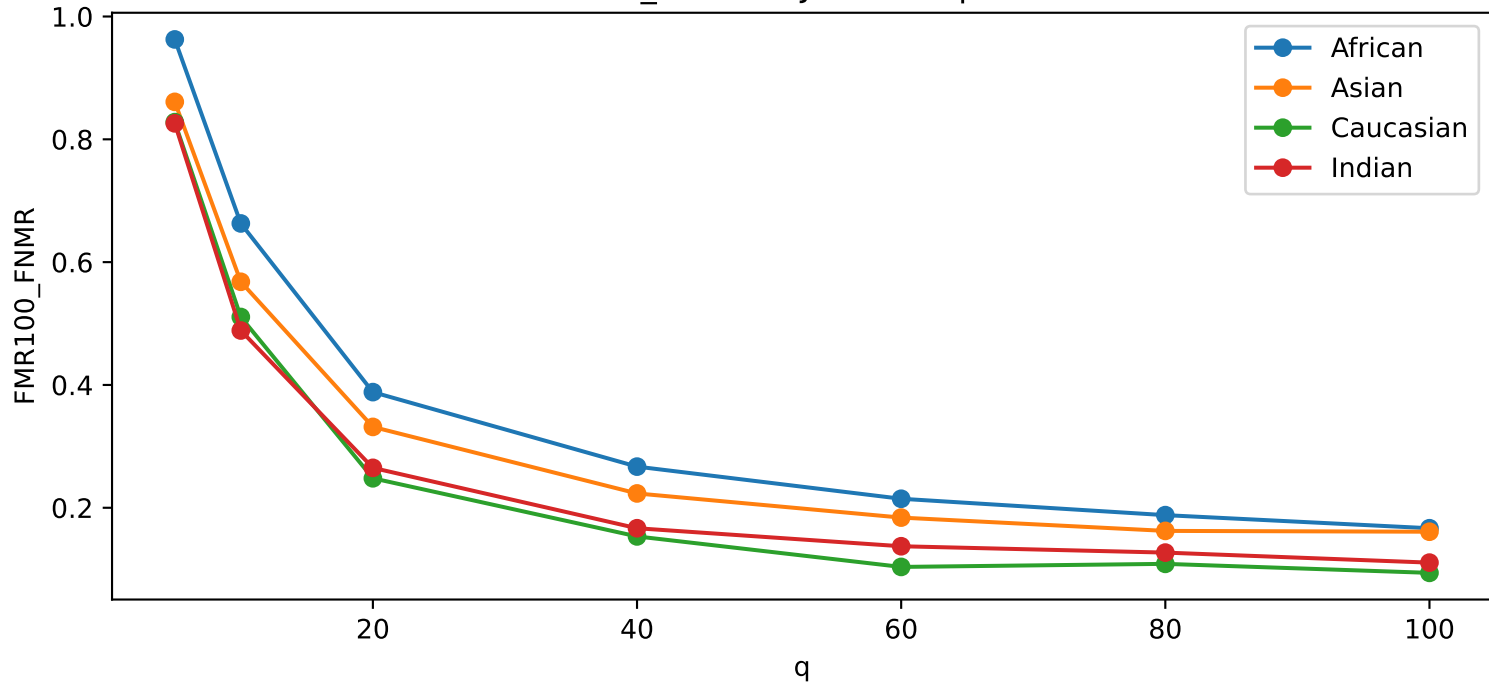
FMR100_FNMR — JPEG Compression
