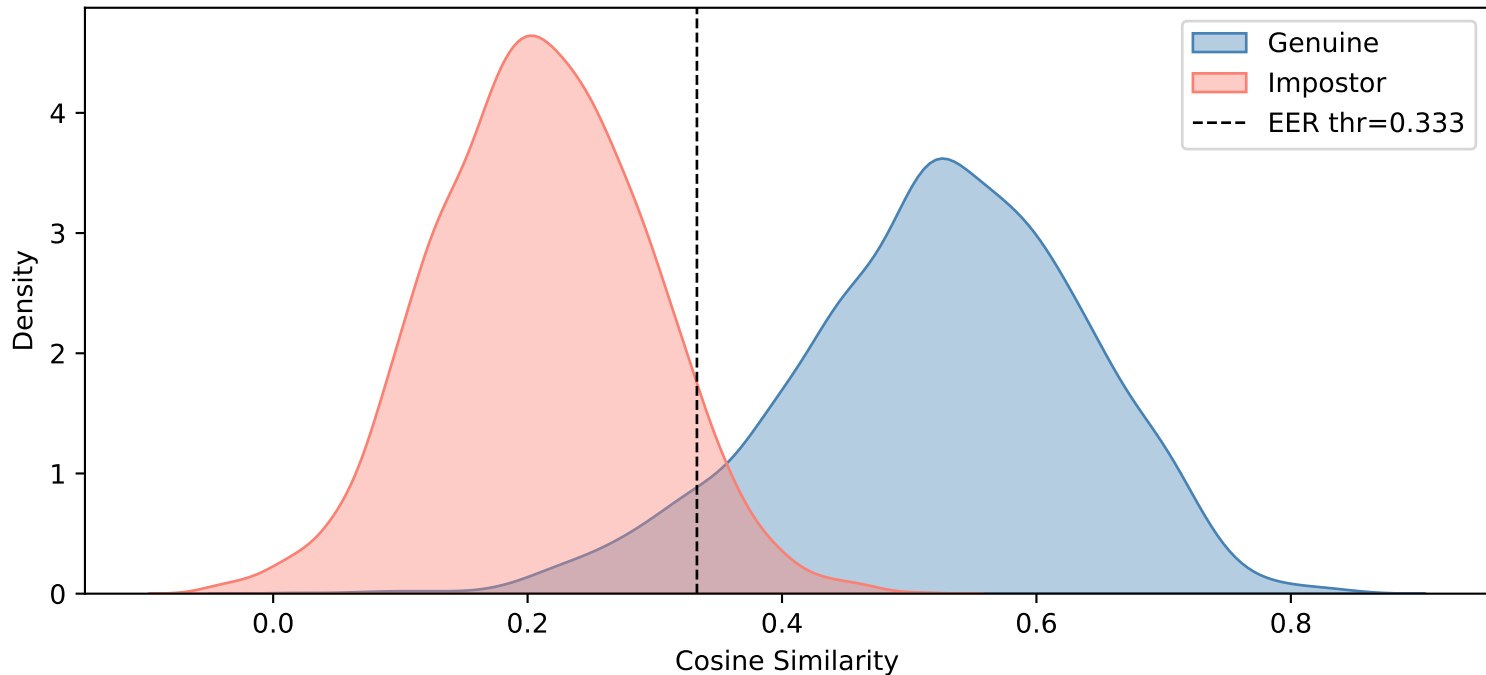
Indian — Contrast ( \alpha=1.5 )
