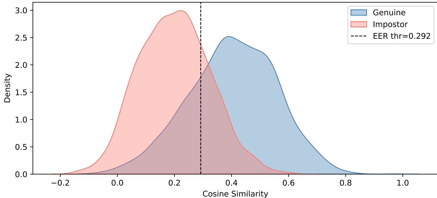
Indian — Gaussian Blur ( \sigma=3.4 )
