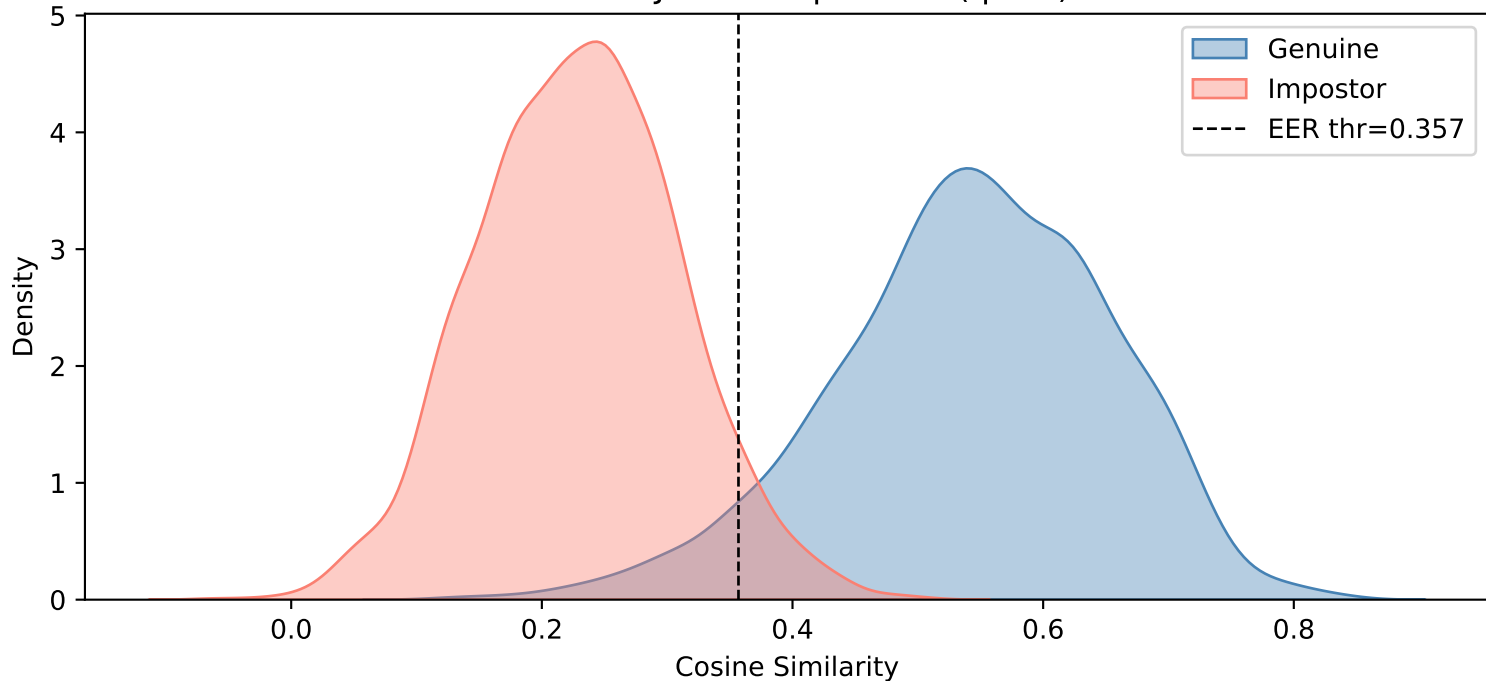
Indian — JPEG Compression (q=80)
