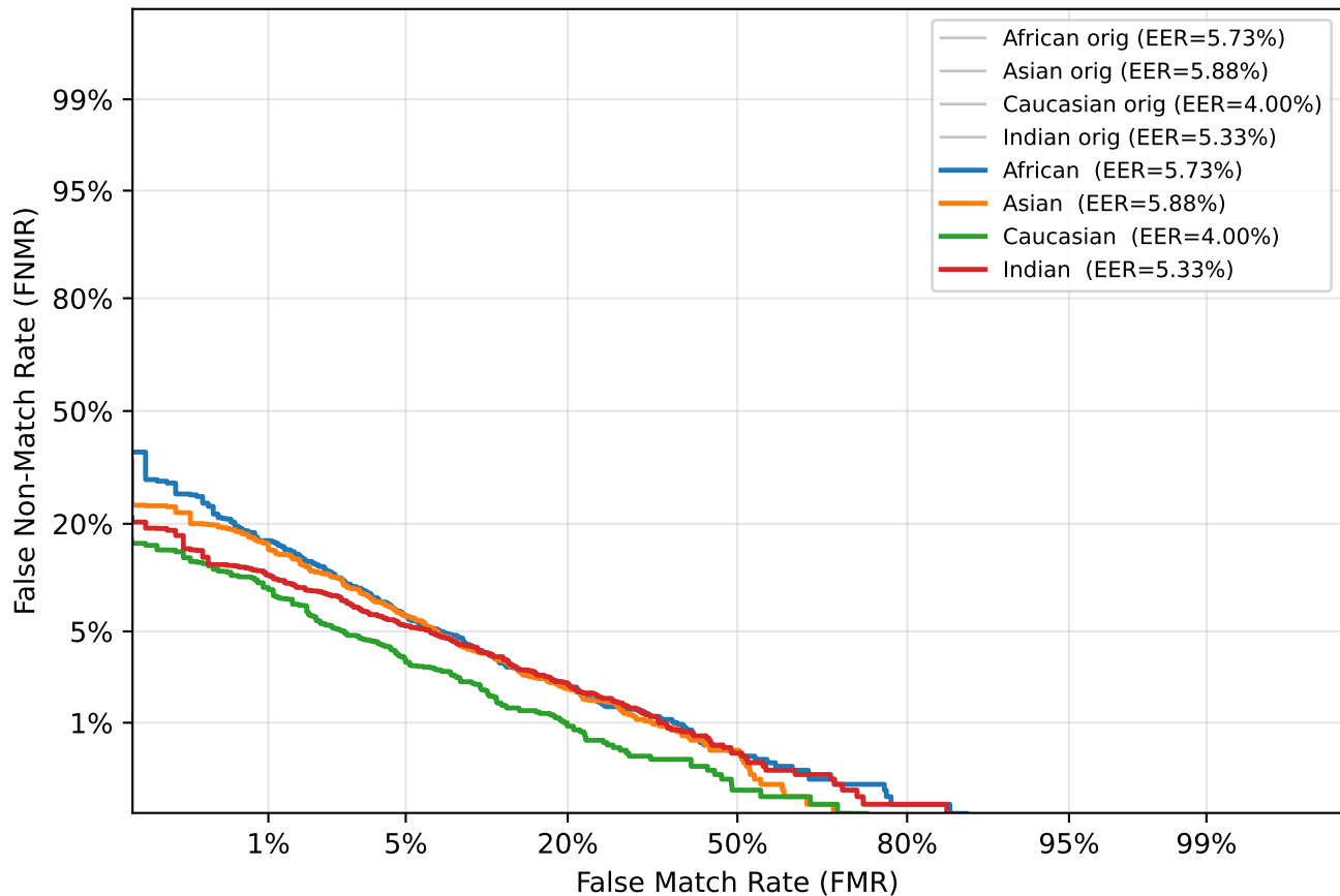
DET — Gaussian Blur ( \sigma=0 )
