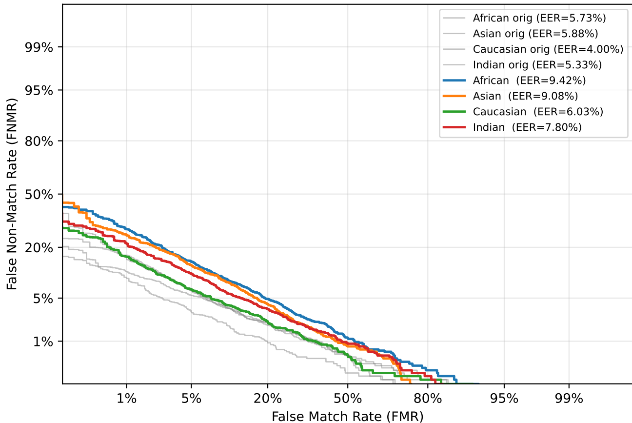
DET — Gaussian Blur ( \sigma=1.4 )
