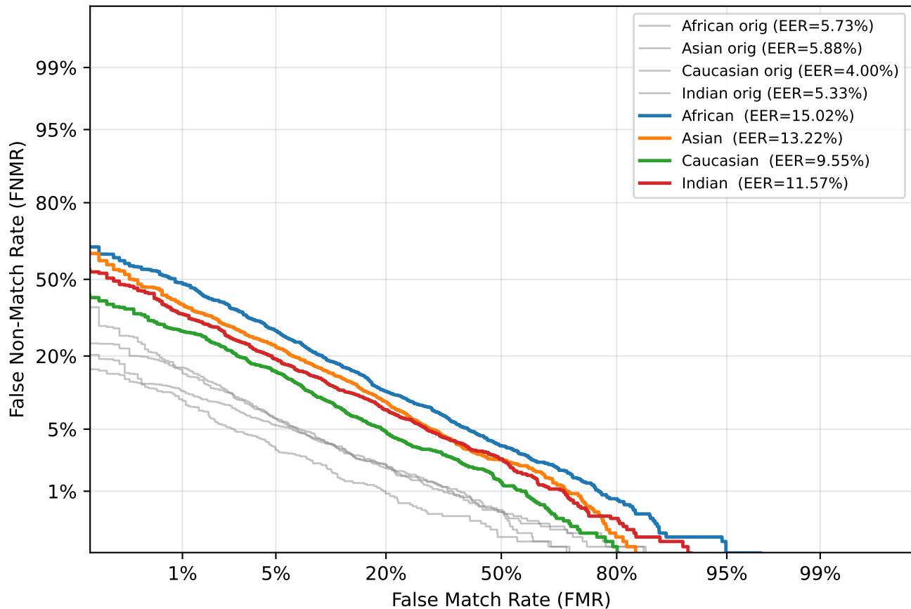
DET — Gaussian Blur ( \sigma=2 )
