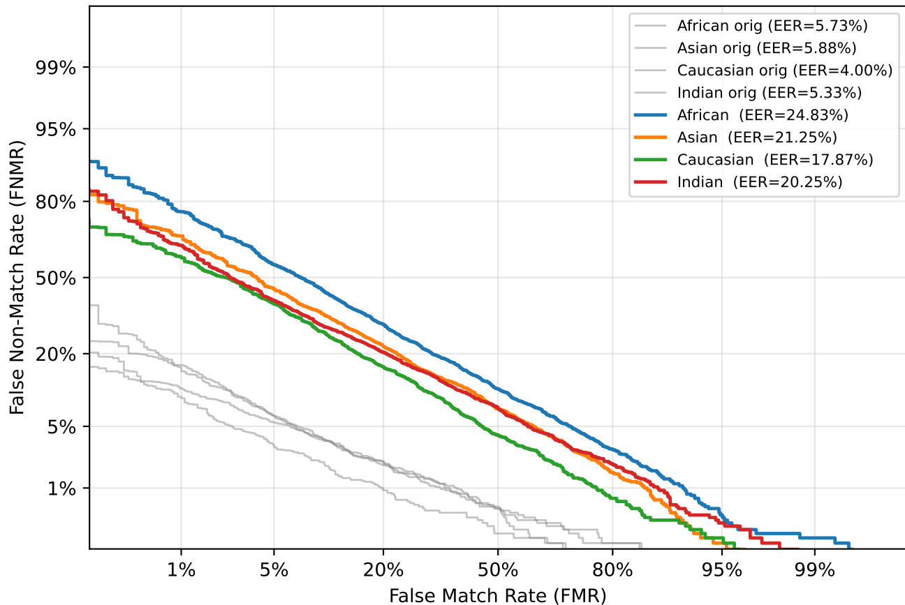
DET — Gaussian Blur ( \sigma=3 )
