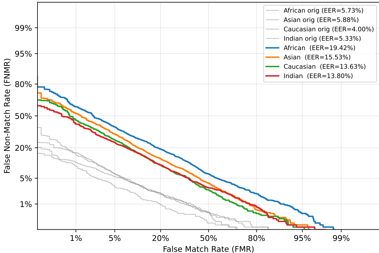
DET — Gaussian Noise ( \sigma=20 )
