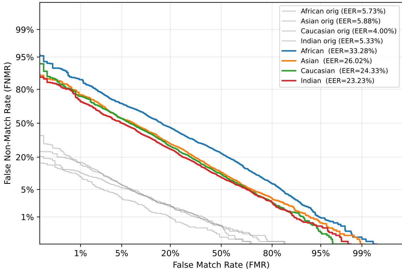
DET — Gaussian Noise ( \sigma=40 )
