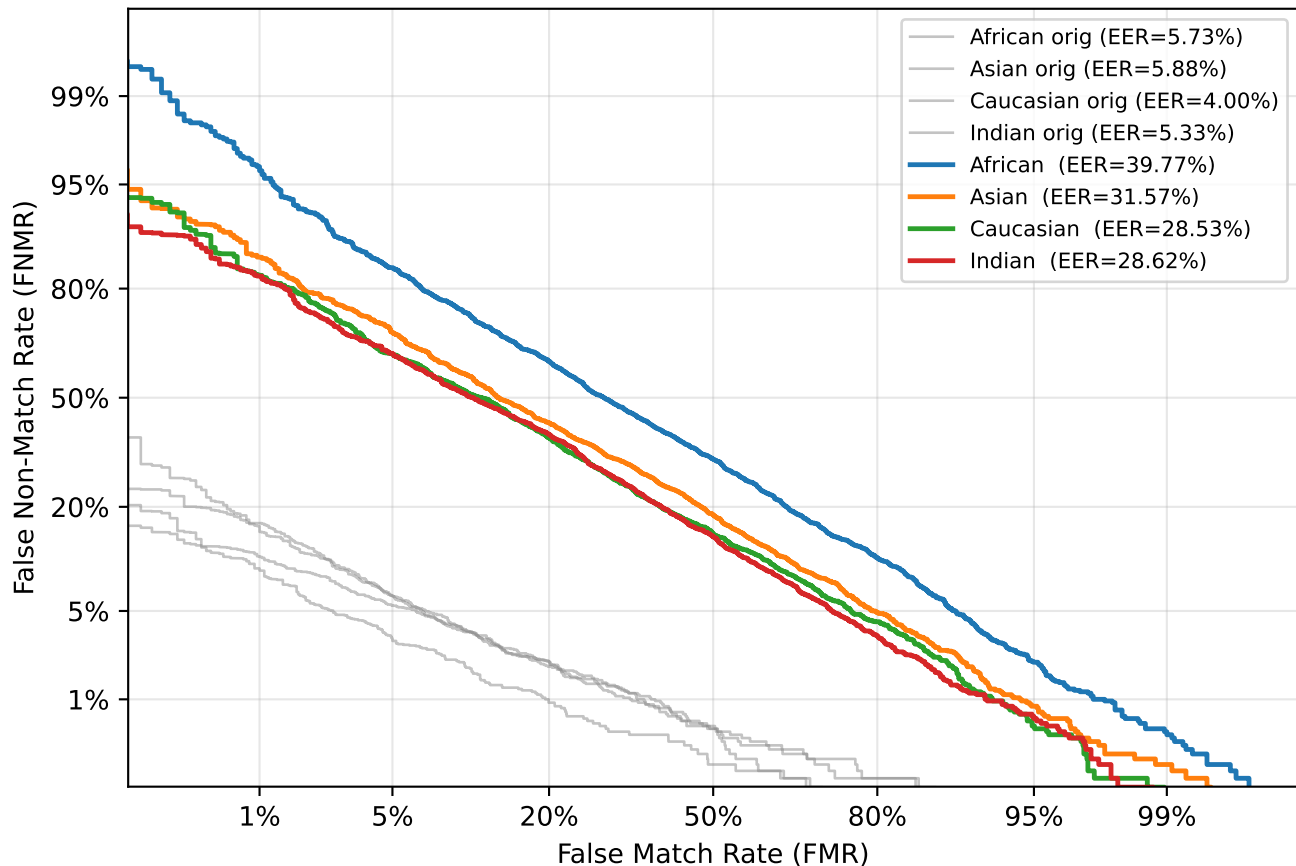
DET — JPEG Compression (q=5)
