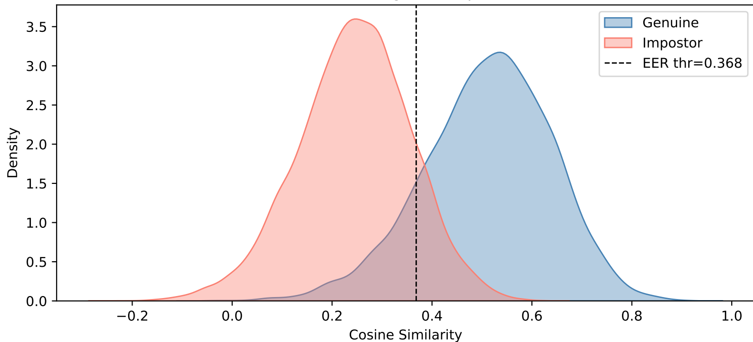
overall — Brightness ( \beta=0.1 )
