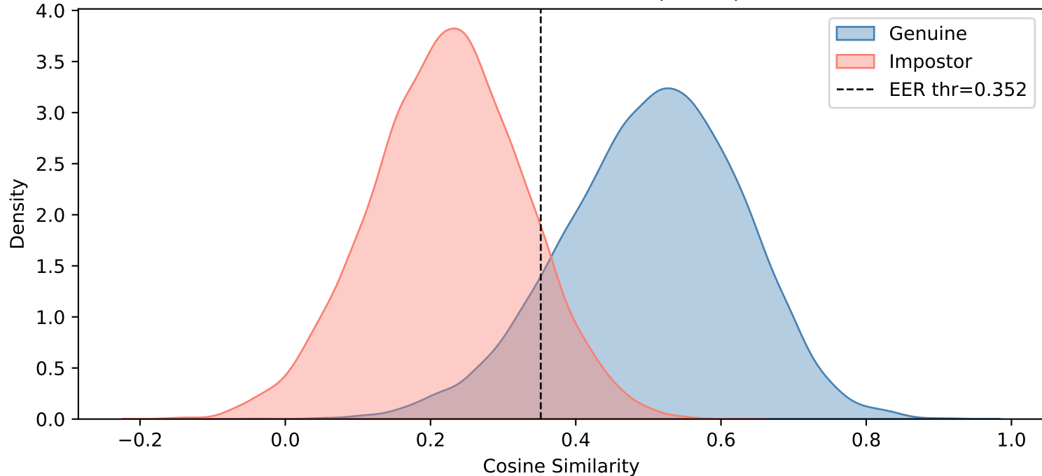
overall — Gaussian Blur ( \sigma=1.8 )
