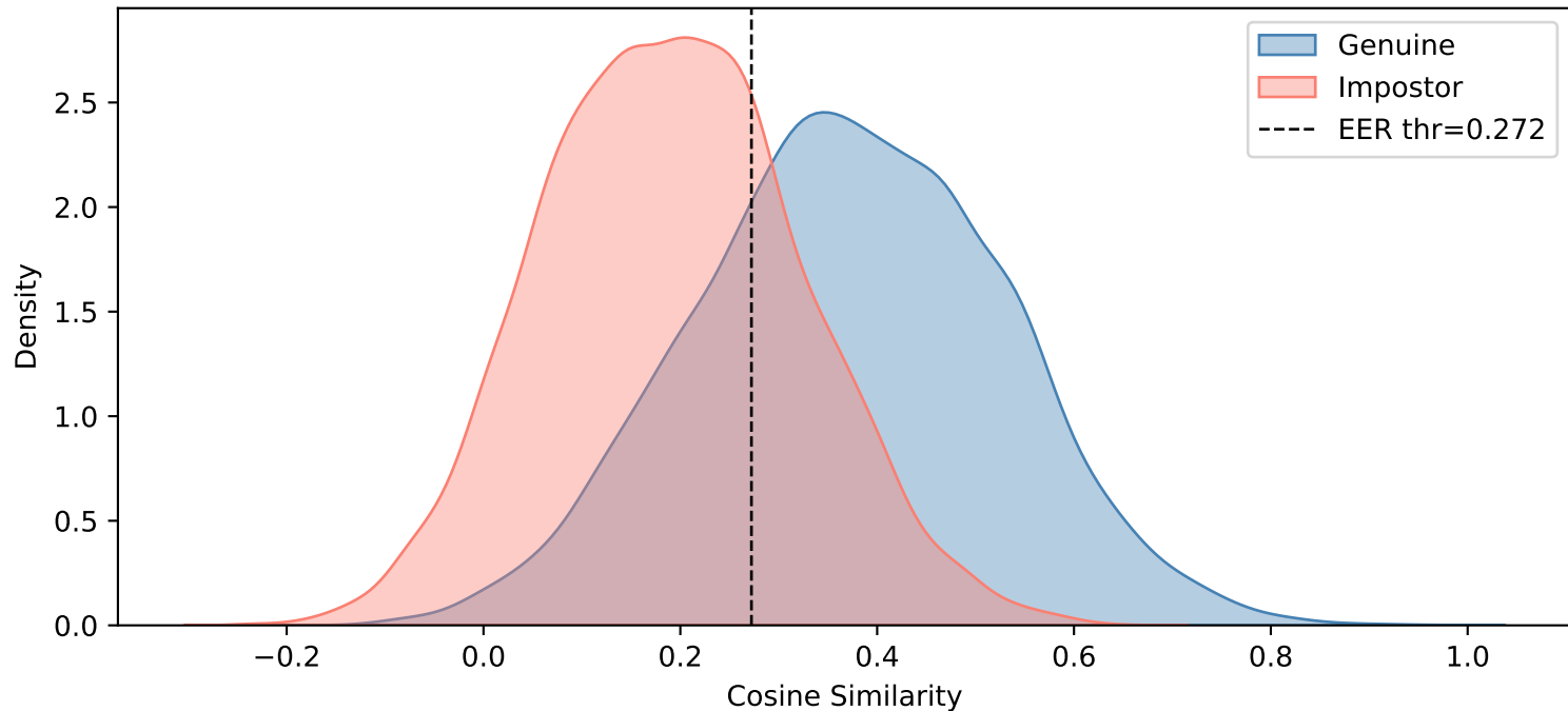
overall — Gaussian Blur ( \sigma=3.6 )
