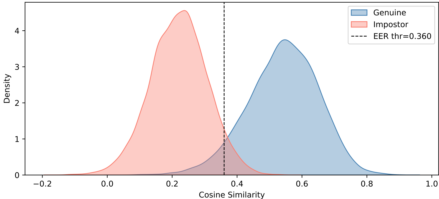
overall — JPEG Compression (q=100)
