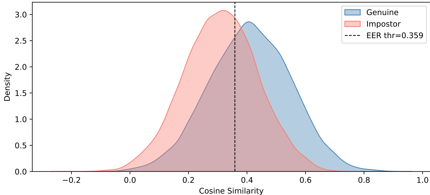
overall — Motion Blur (k=21)
