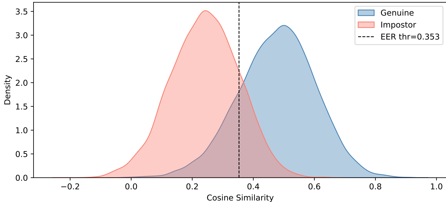
overall — Motion Blur (k=9)
